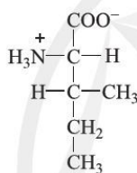
d) Amino acid
