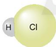
a) Hydrogen chloride
