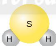
b) Hydrogen sulfide
