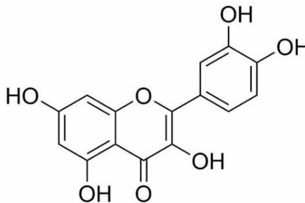
quercetin
